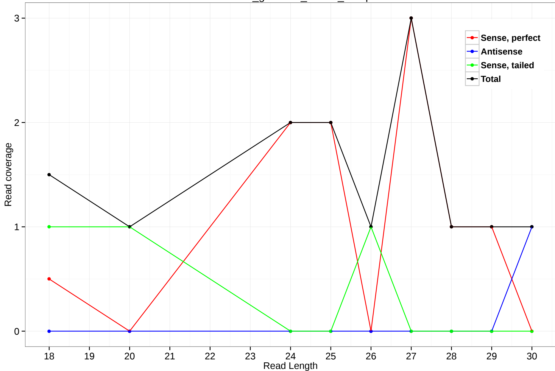
rheMac3_genscan_chr4.2_14.3p
