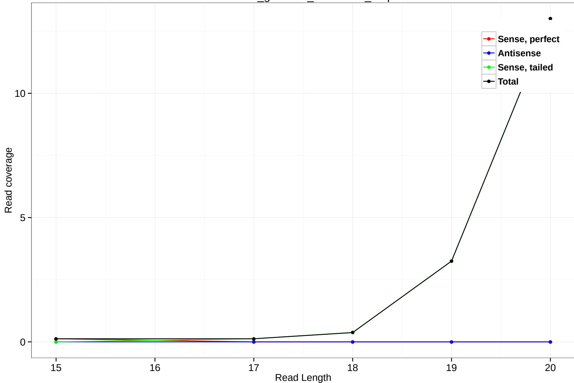
rheMac3_genscan_chr4.2942_2.3p
