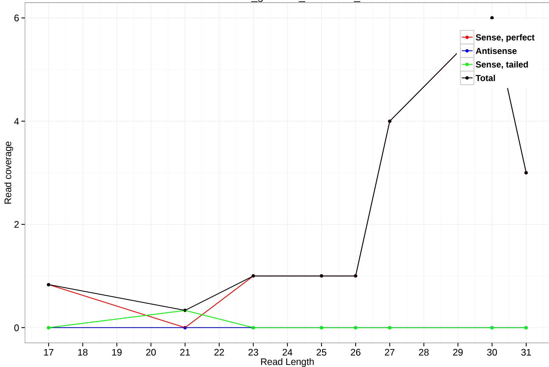
rheMac3_genscan_chr4.2904_6
