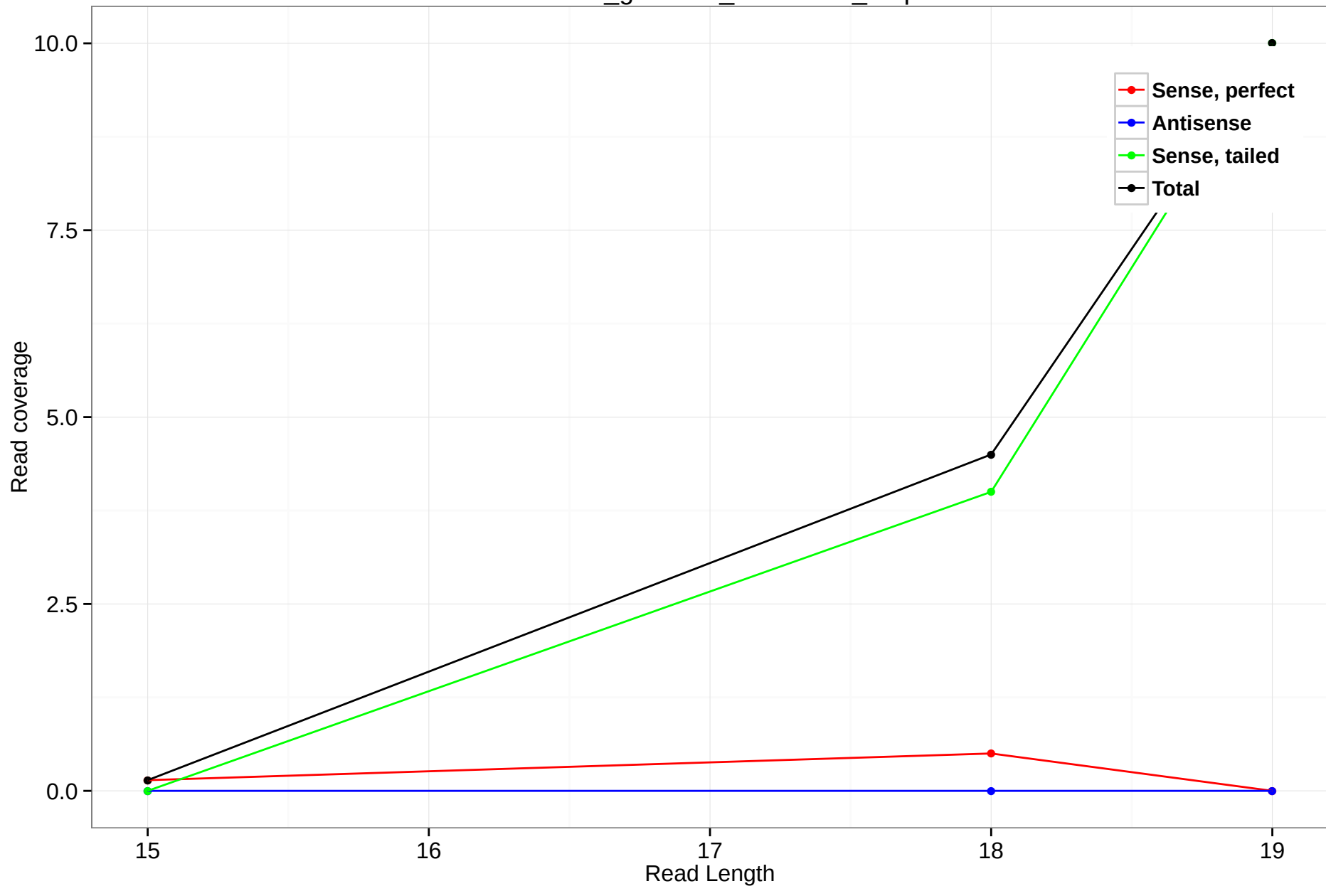
rheMac3_genscan_chr4.2860_1.3p
