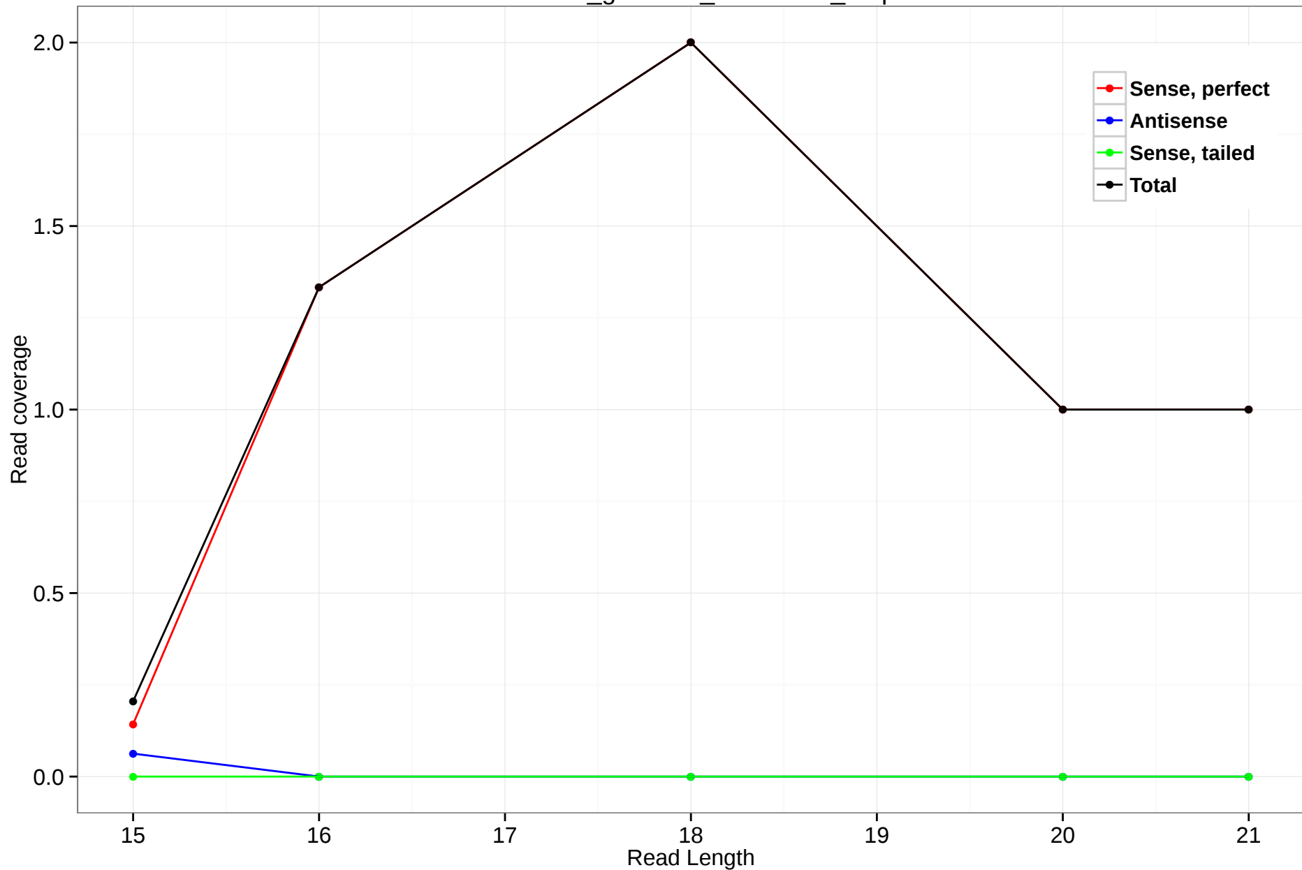
rheMac3_genscan_chr4.2851_0.3p
