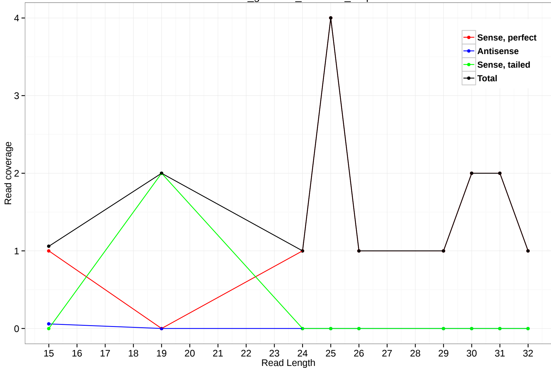
rheMac3_genscan_chr4.280_6.3p
