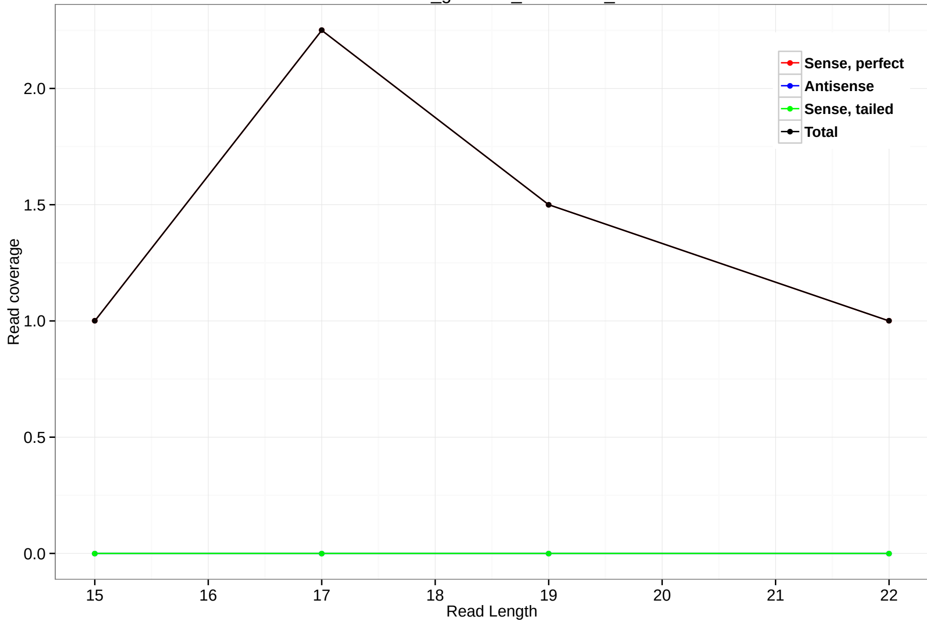
rheMac3_genscan_chr4.2680_1
