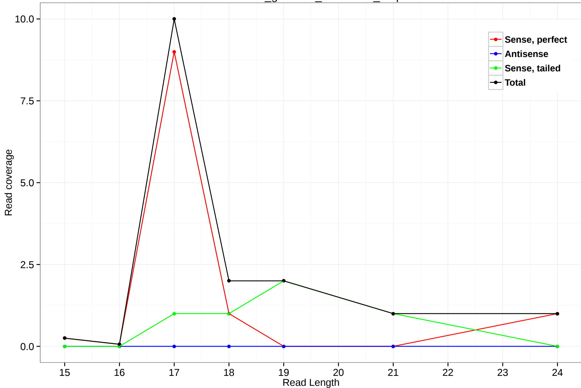
rheMac3_genscan_chr4.2633_1.3p
