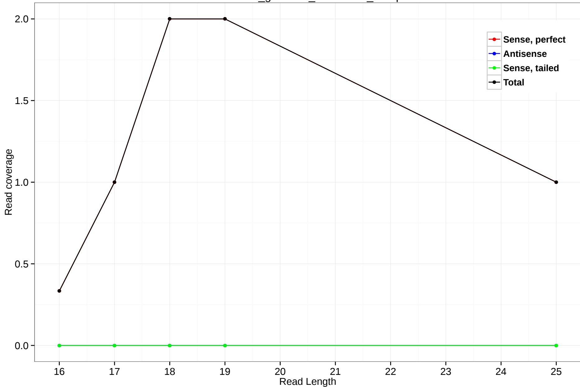
rheMac3_genscan_chr4.2510_14.5p
