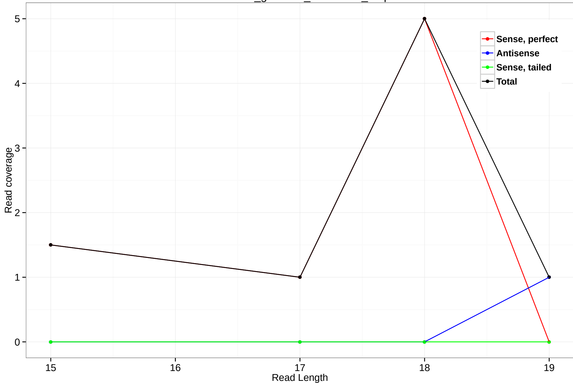
rheMac3_genscan_chr4.2451_5.3p
