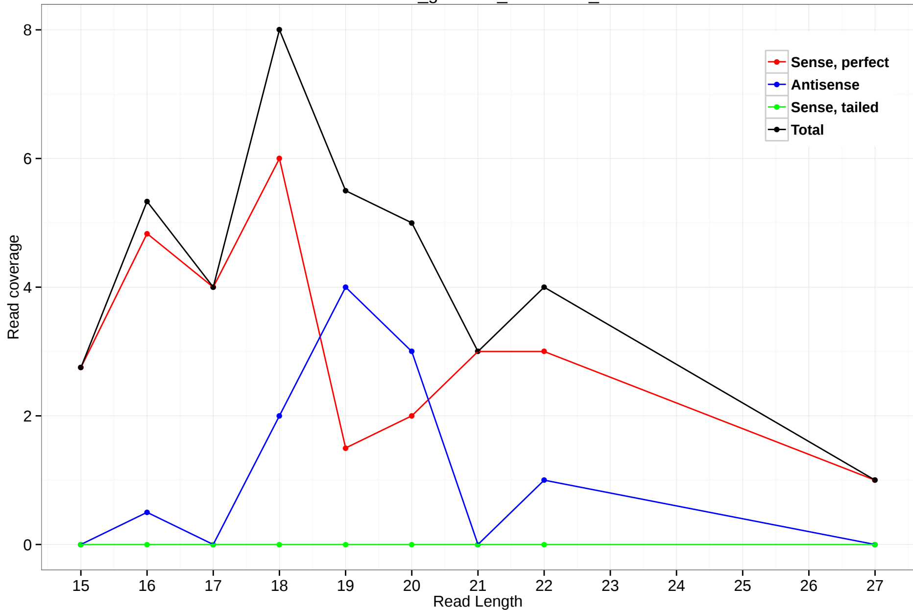
rheMac3_genscan_chr4.2298_5
