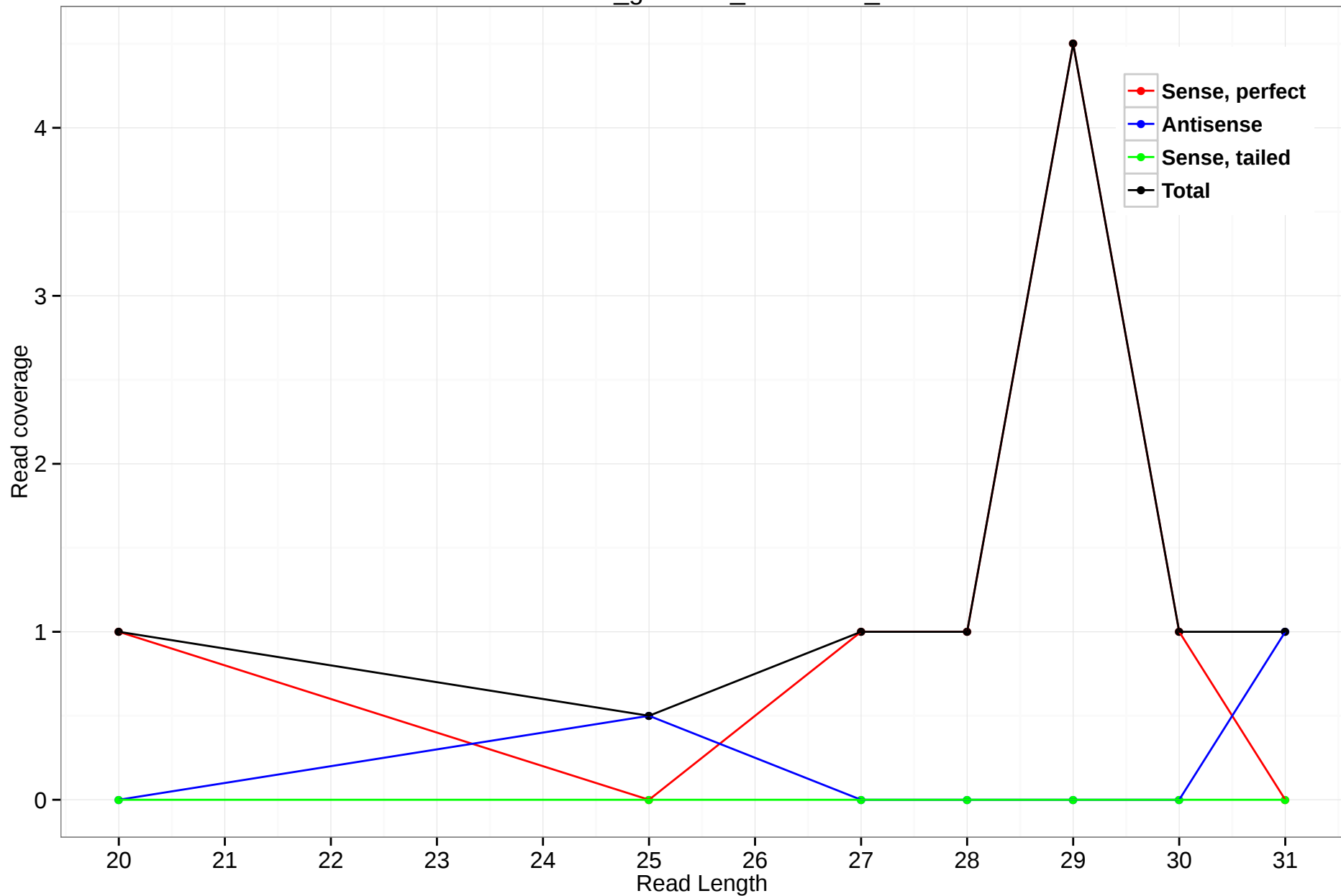
rheMac3_genscan_chr4.2205_5
