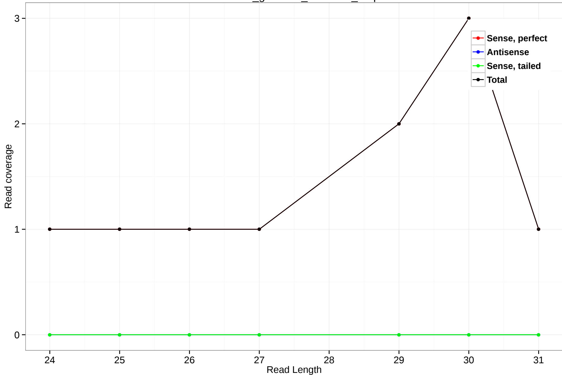
rheMac3_genscan_chr4.213_1.3p
