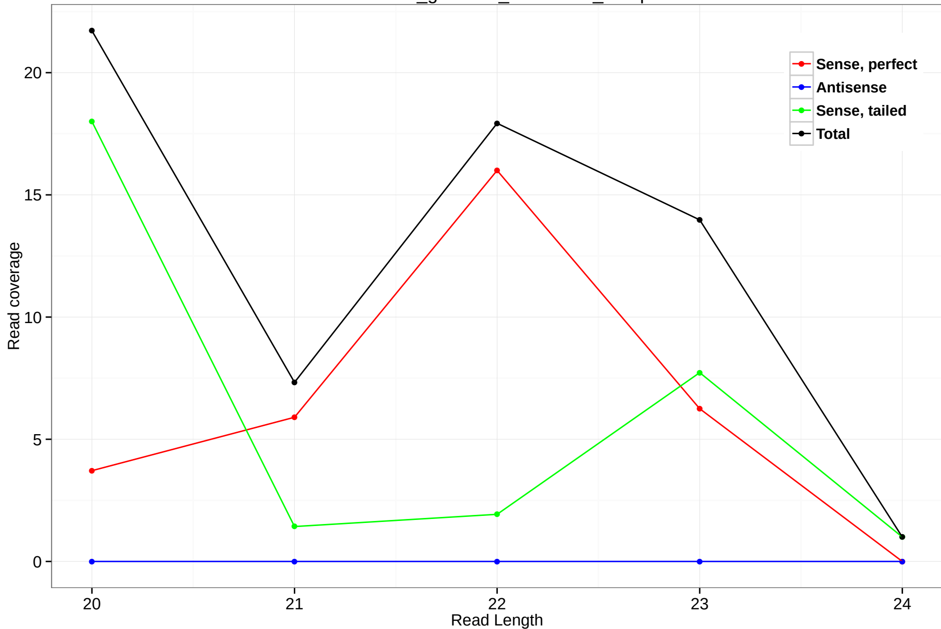
rheMac3_genscan_chr4.2060_12.3p
