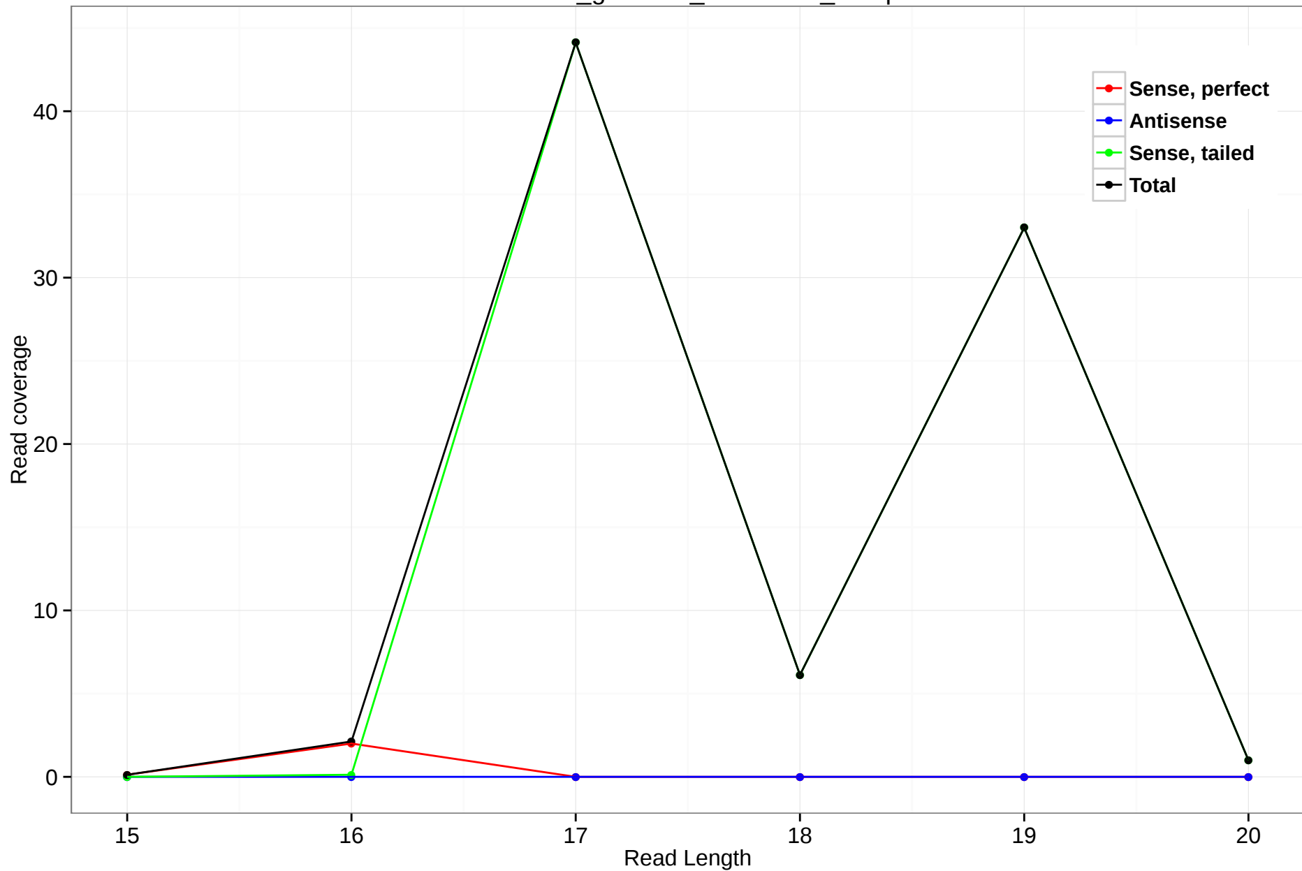
rheMac3_genscan_chr4.1857_11.5p
