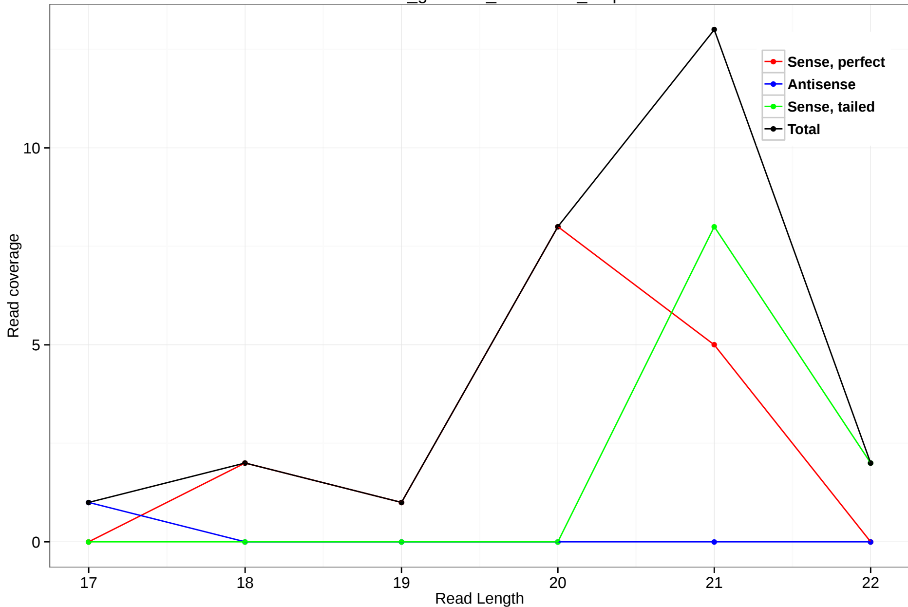
rheMac3_genscan_chr4.1829_6.3p
