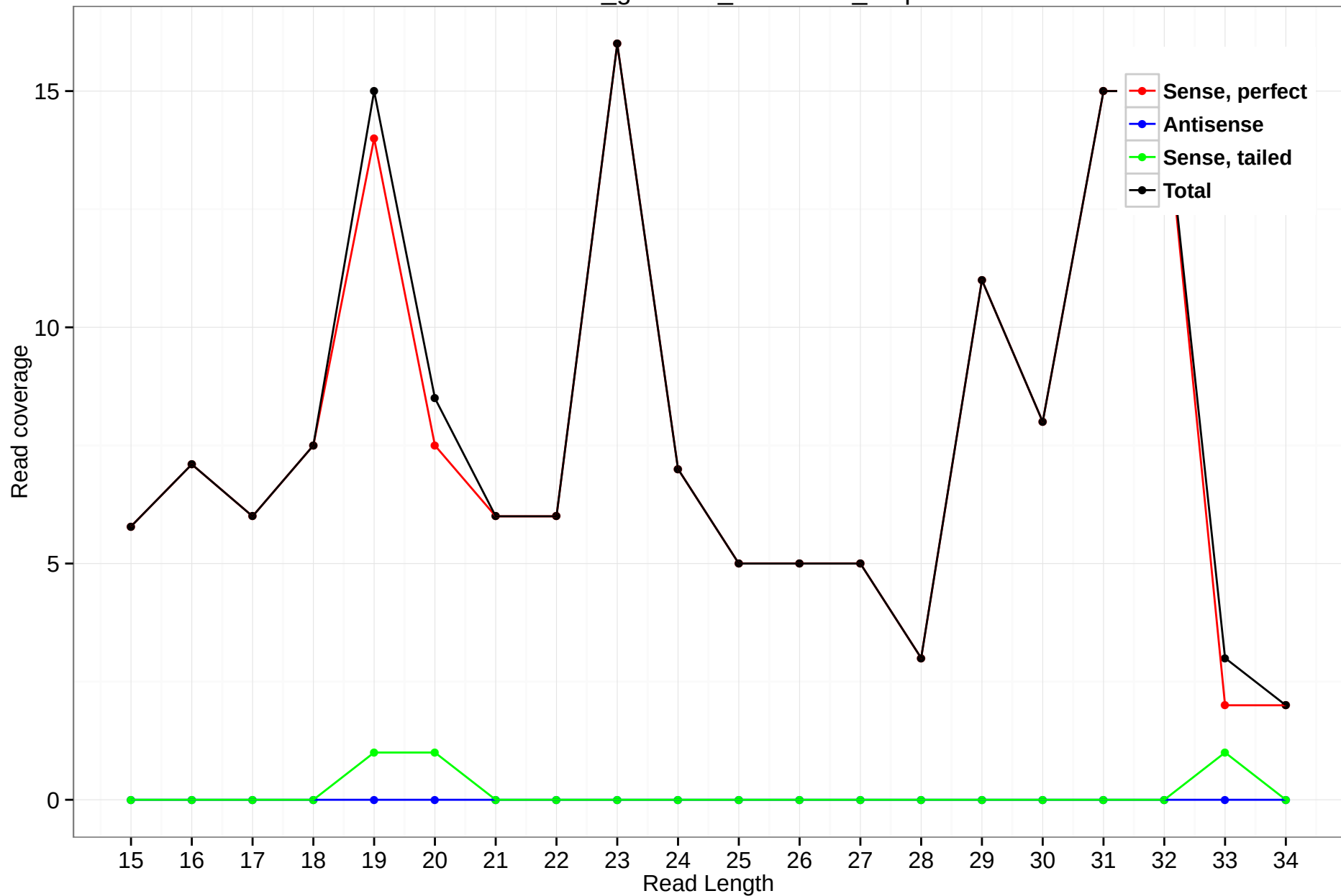
rheMac3_genscan_chr4.1780_3.3p
