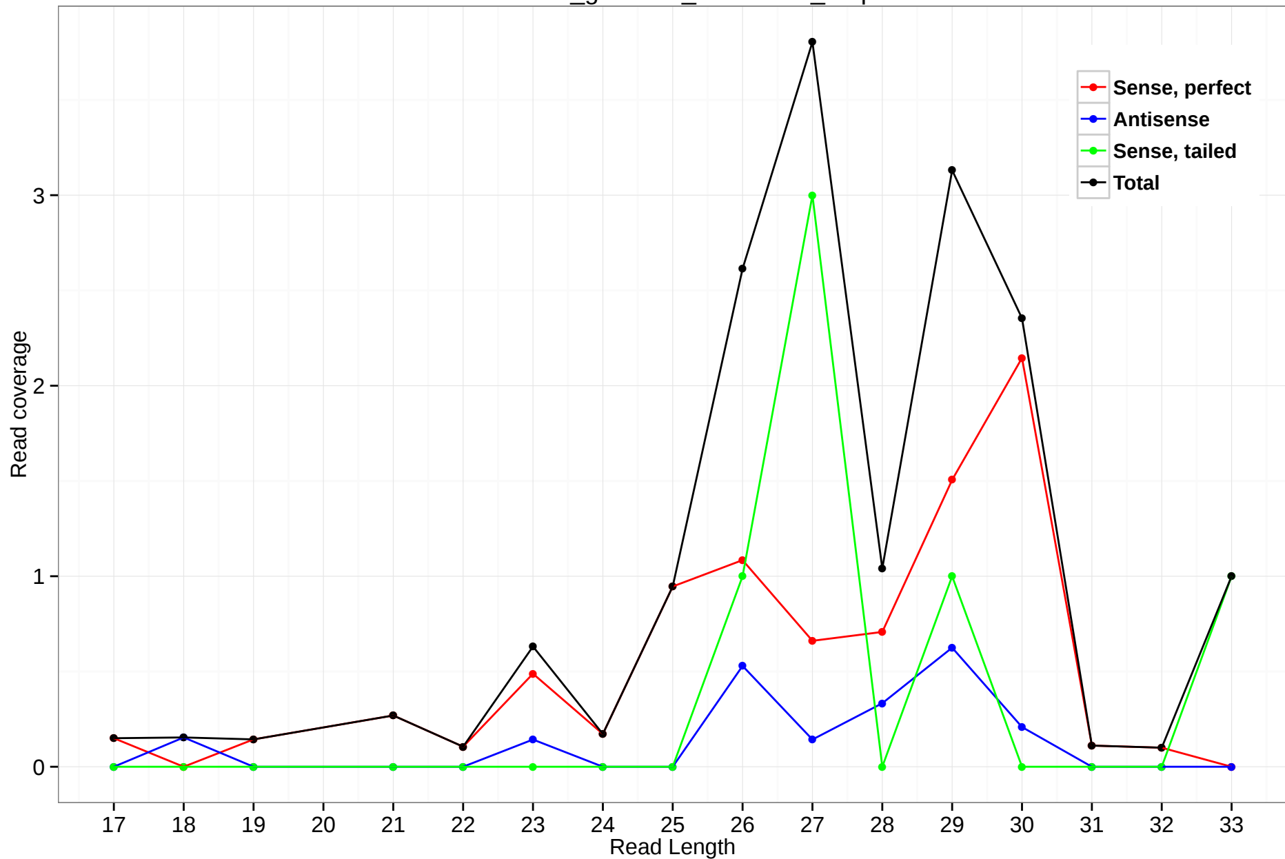
rheMac3_genscan_chr4.1548_7.3p
