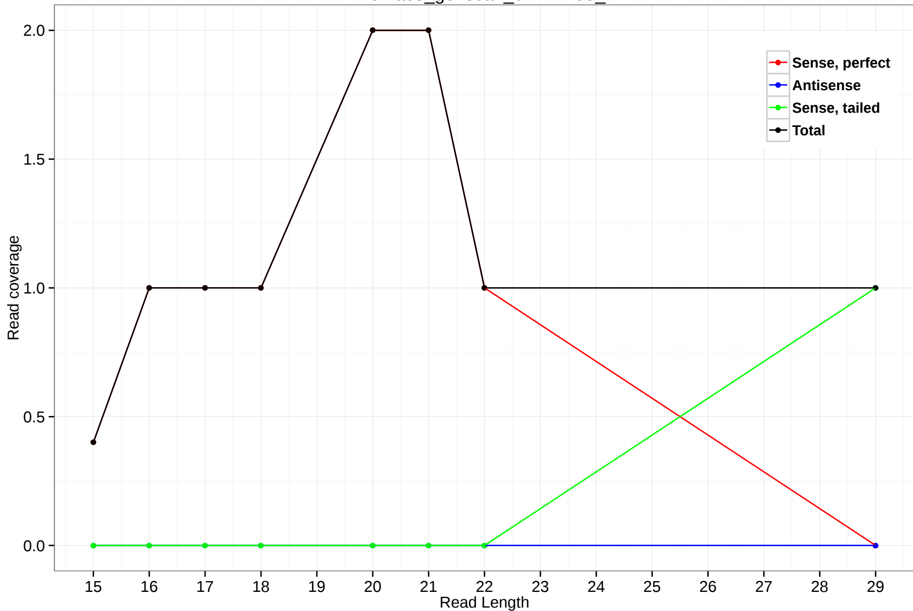
rheMac3_genscan_chr4.1495_1
