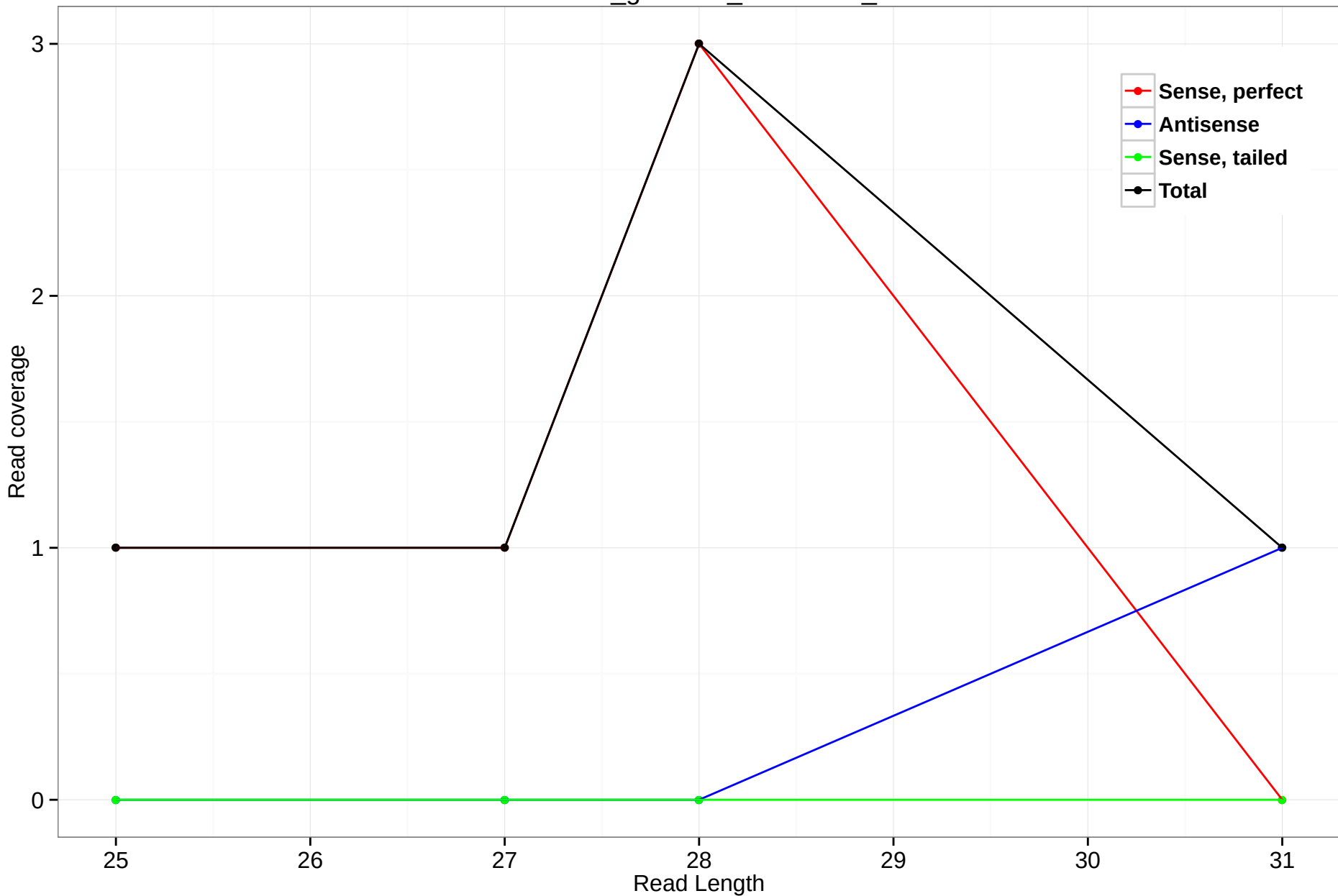
rheMac3_genscan_chr4.1428_7
