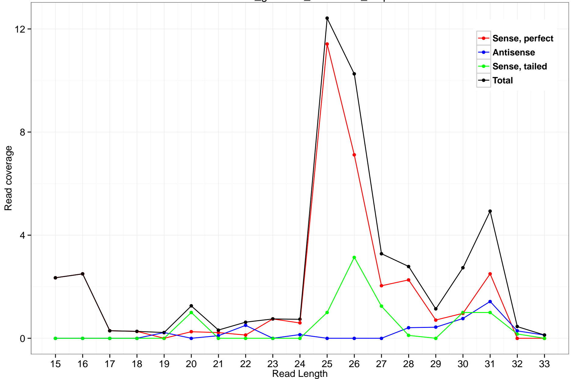
rheMac3_genscan_chr4.1359_0.5p
