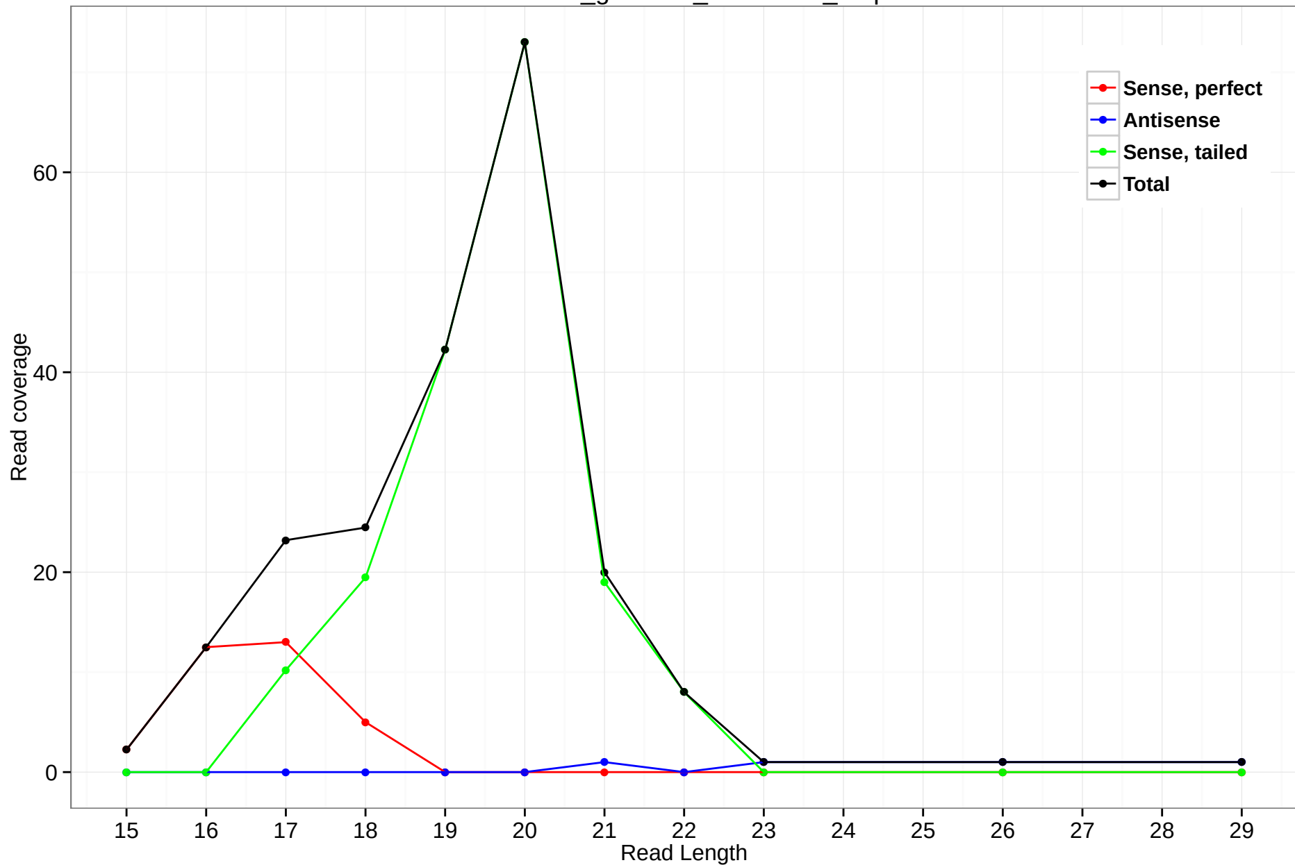
rheMac3_genscan_chr4.1239_0.3p
