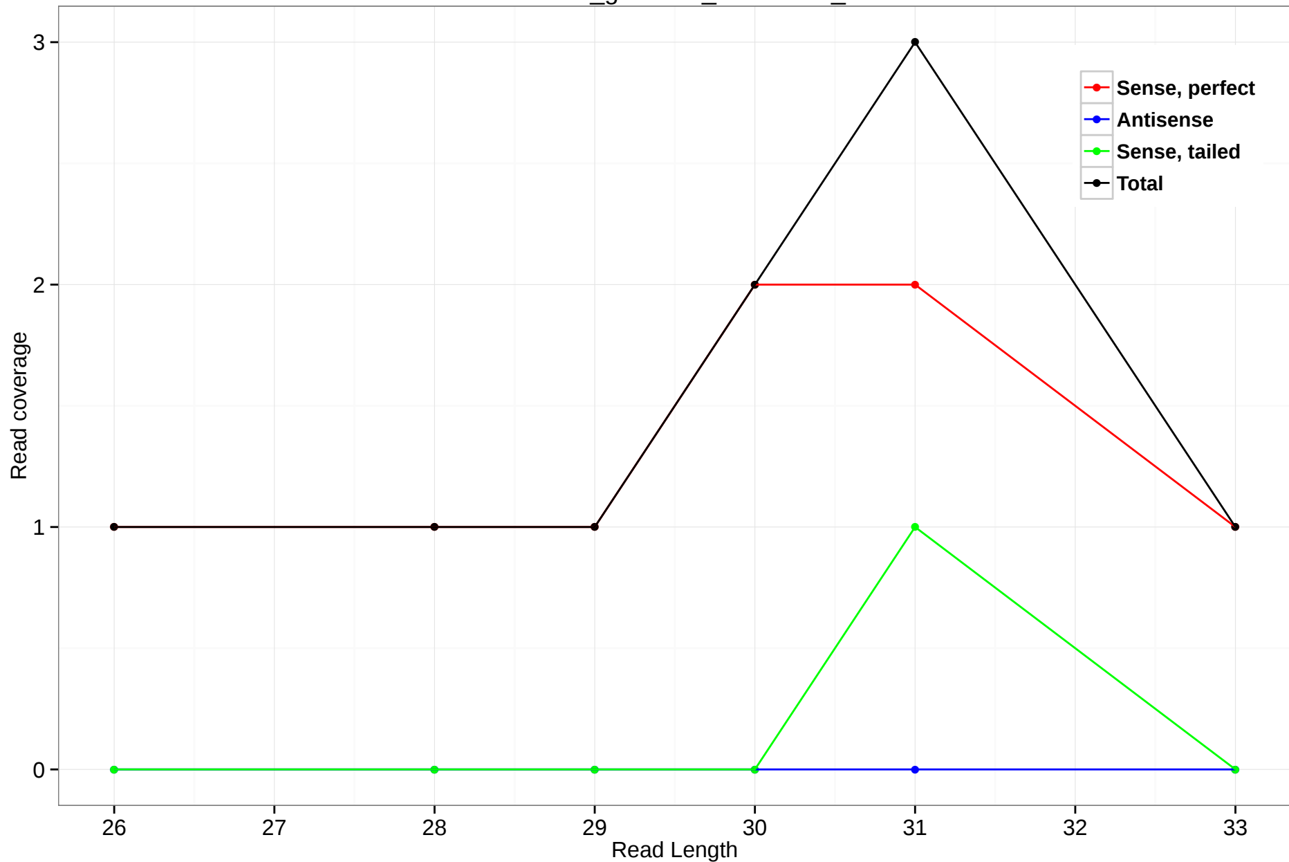
rheMac3_genscan_chr4.1180_2
