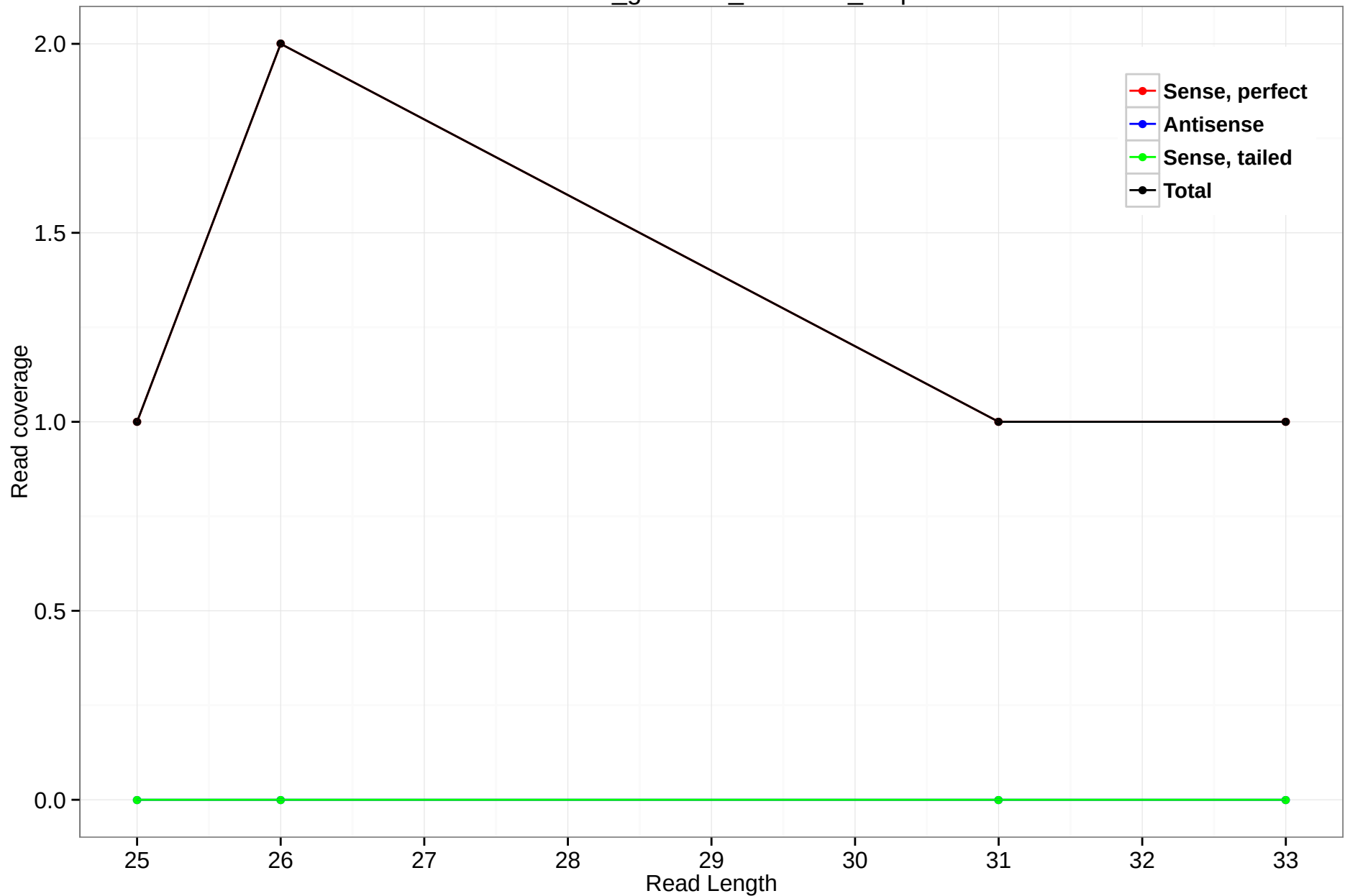
rheMac3_genscan_chr4.117_3.3p
