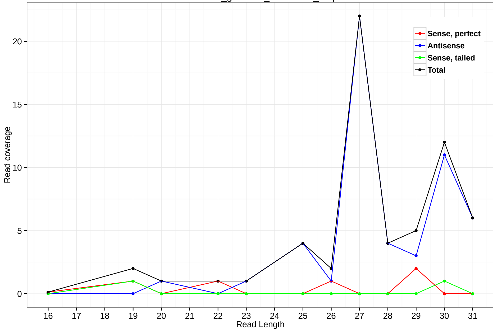
rheMac3_genscan_chr4.1115_1.5p
