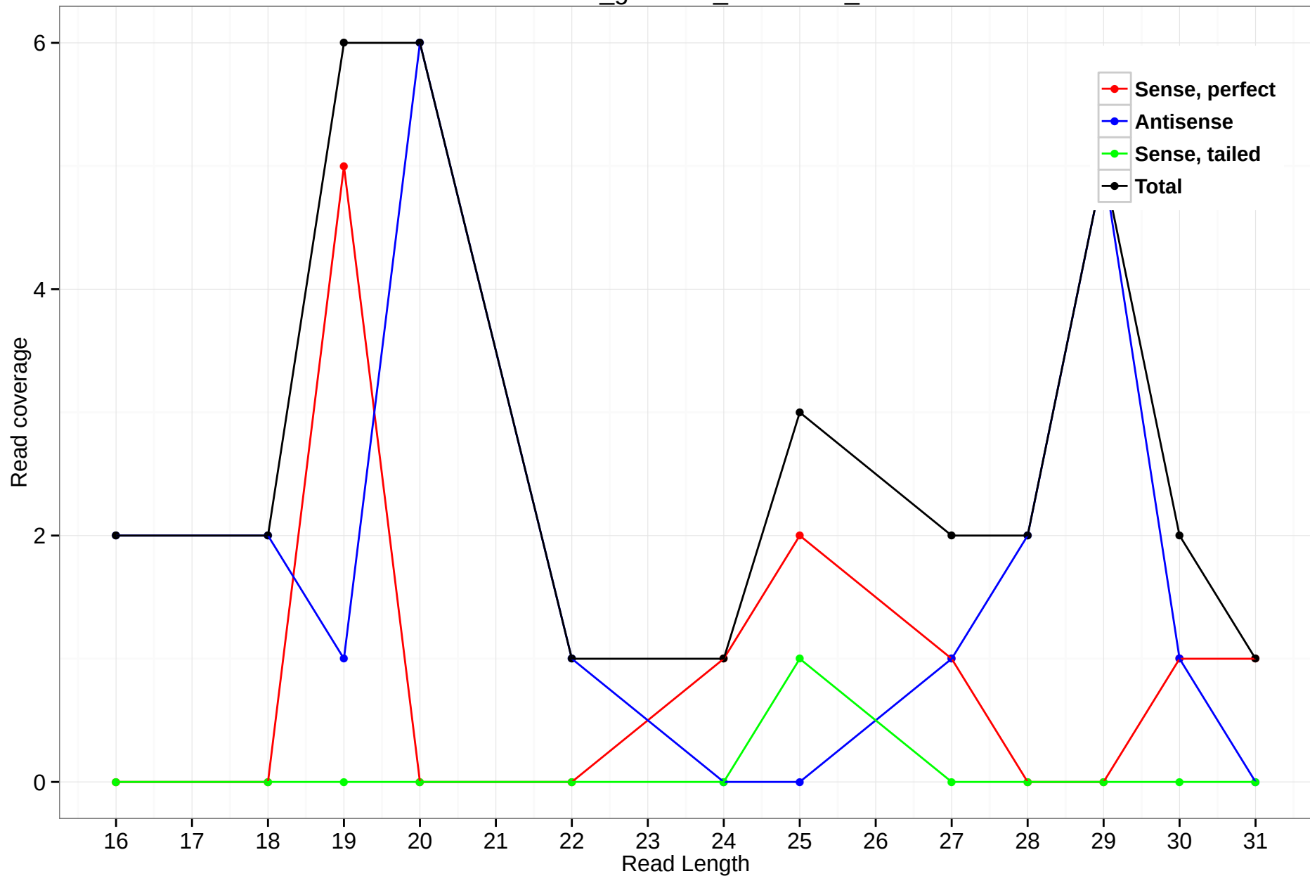
rheMac3_genscan_chr4.1089_2
