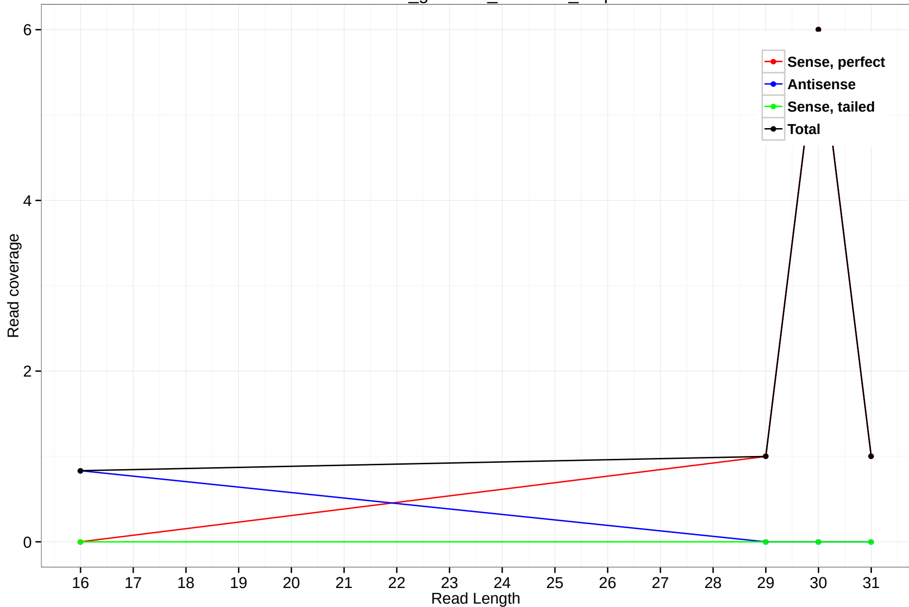
rheMac3_genscan_chr4.102_4.5p
