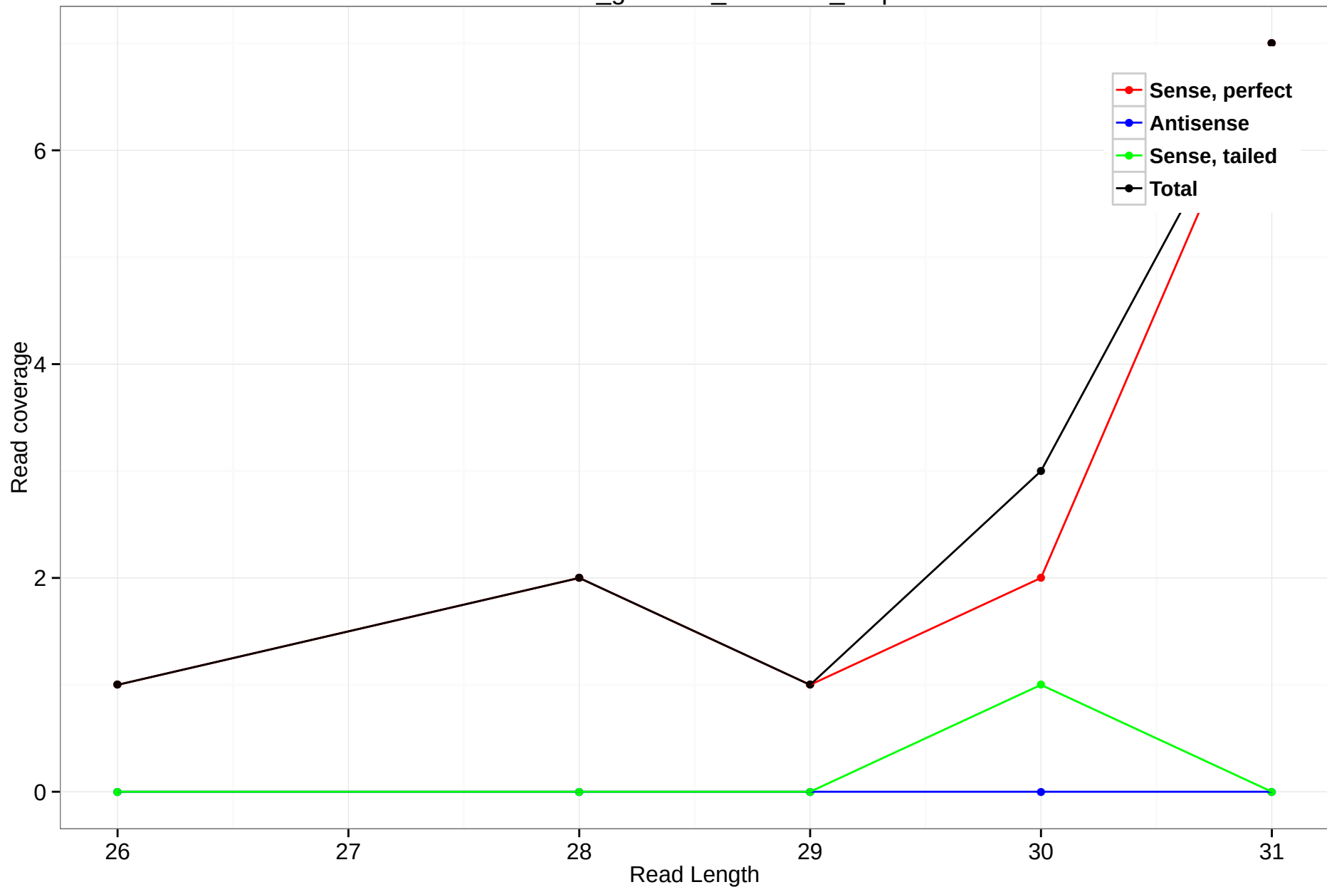
rheMac3_genscan_chr4.102_2.3p
