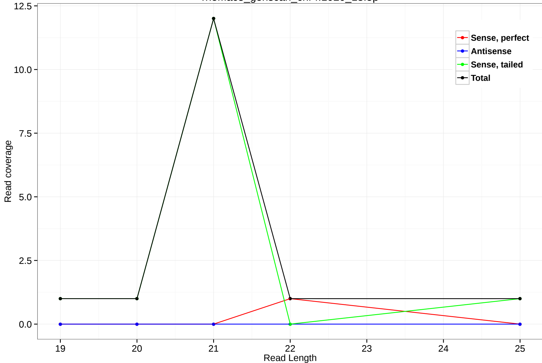
rheMac3_genscan_chr4.1020_18.5p
