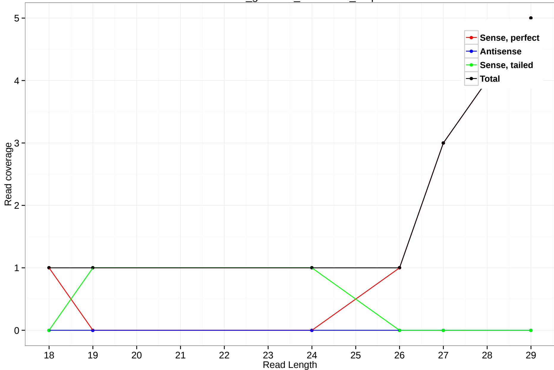
rheMac3_genscan_chr4.1014_8.5p
