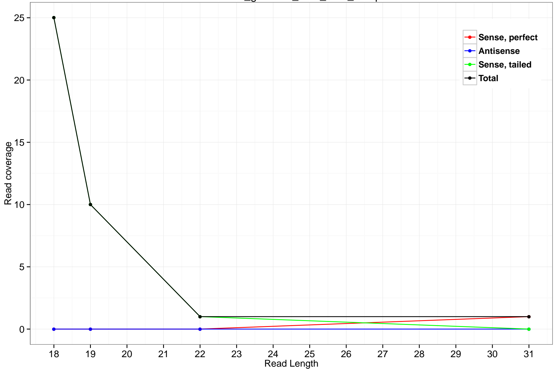
rheMac3_genscan_chr3_98.7_14.5p
