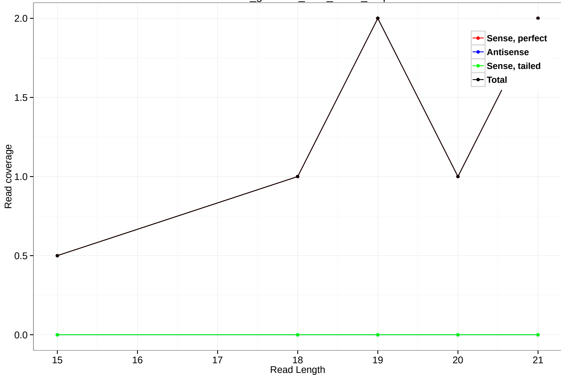
rheMac3_genscan_chr3_98.26_0.5p
