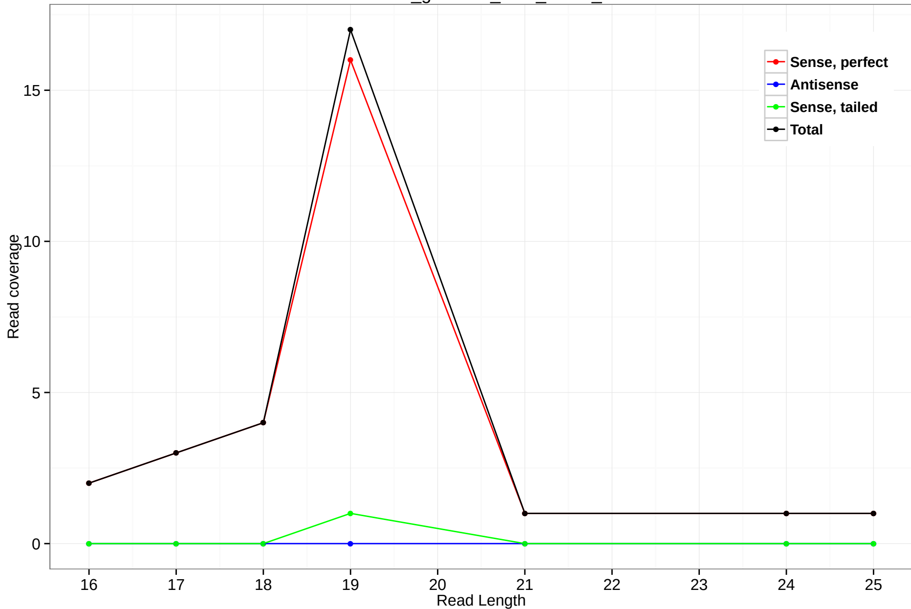
rheMac3_genscan_chr3_98.12_10
