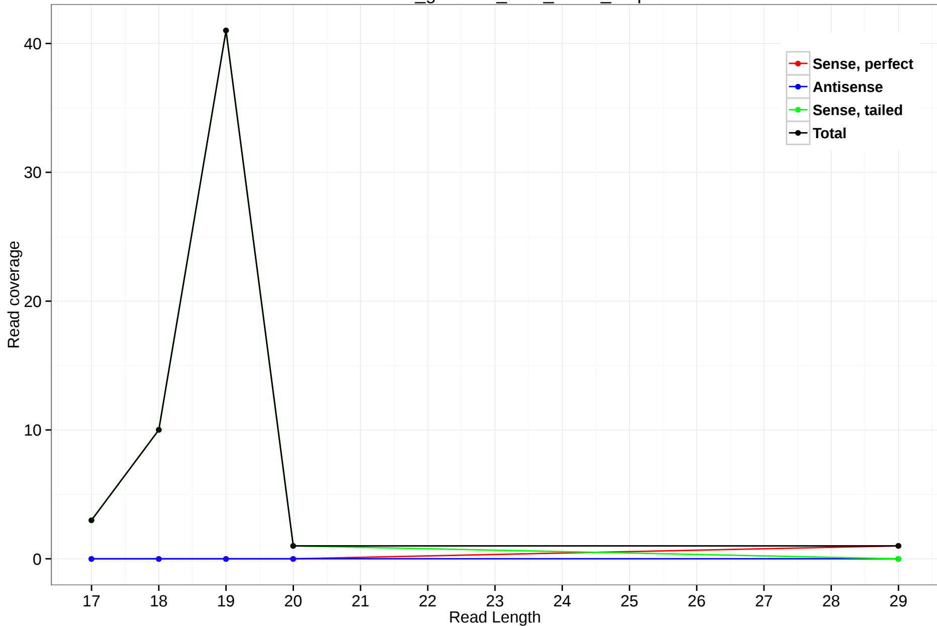
rheMac3_genscan_chr3_96.16_6.5p
