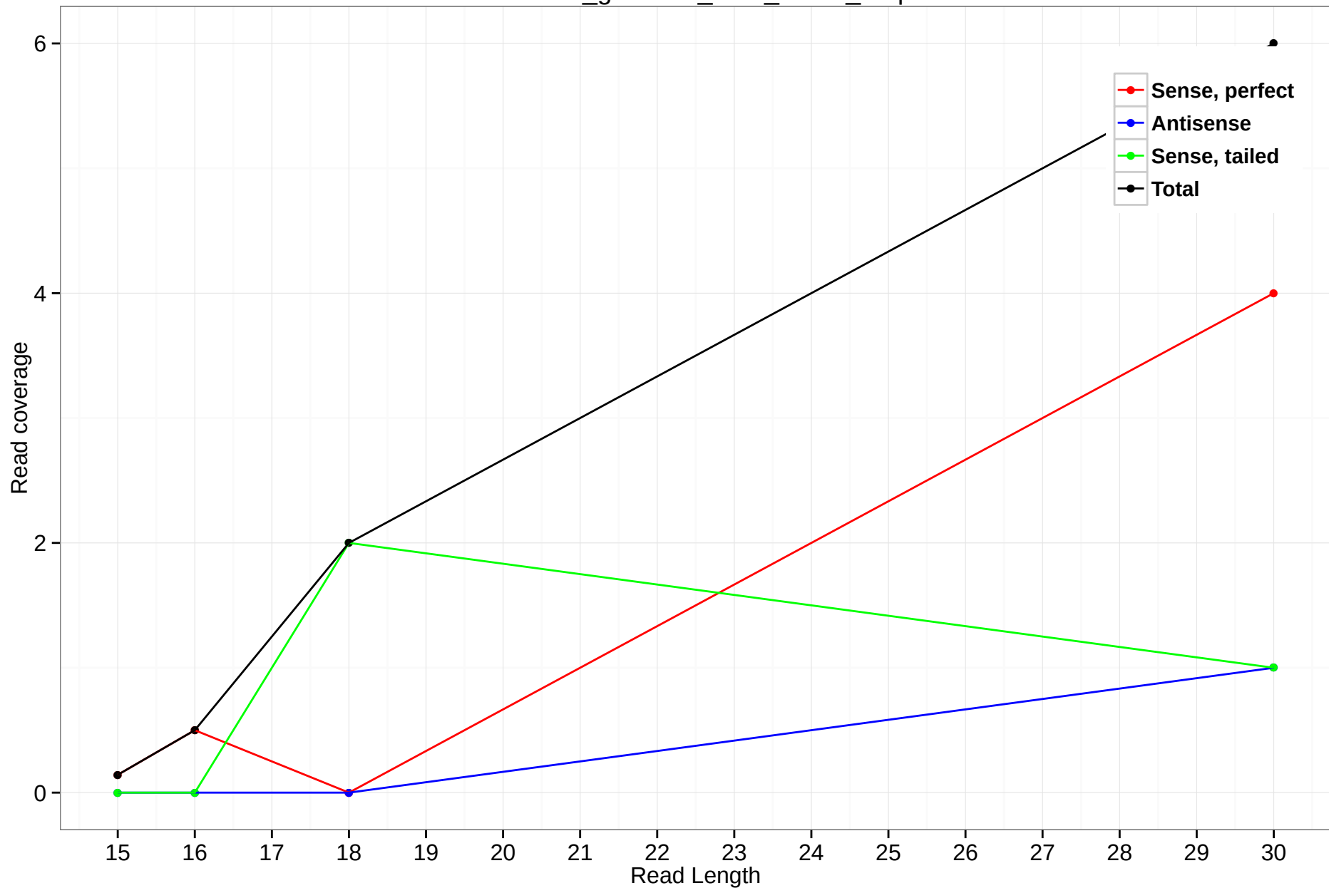
rheMac3_genscan_chr3_96.15_0.3p
