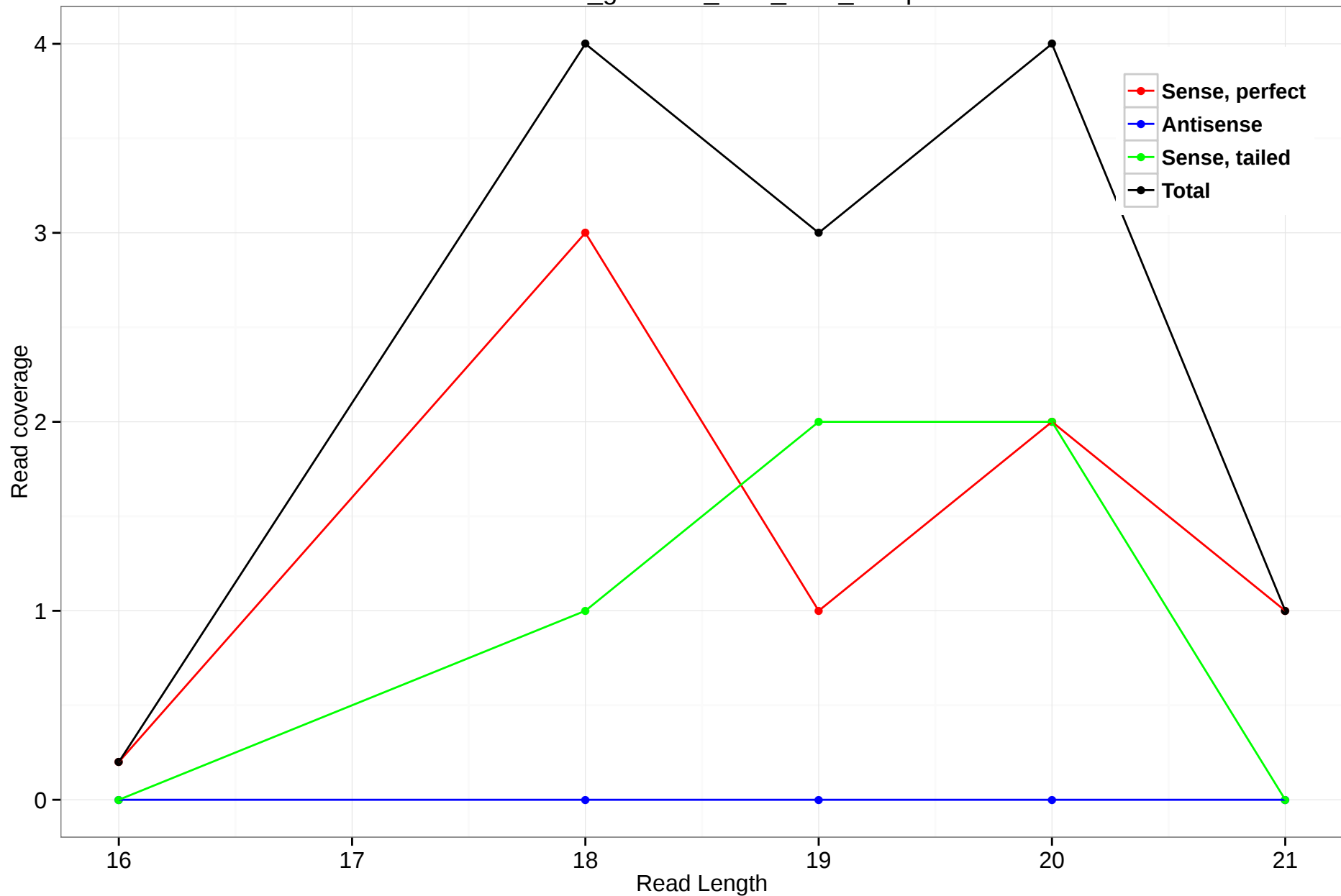
rheMac3_genscan_chr3_94.2_12.5p
