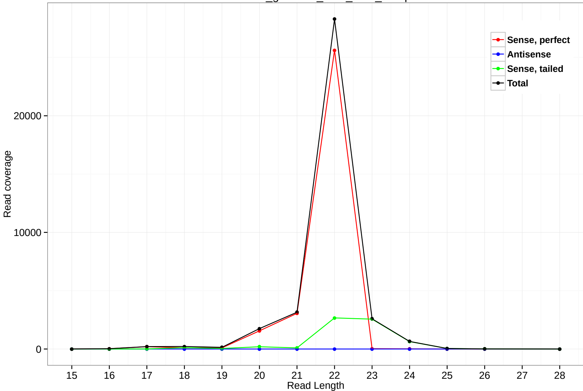
rheMac3_genscan_chr3_91.9_11.3p
