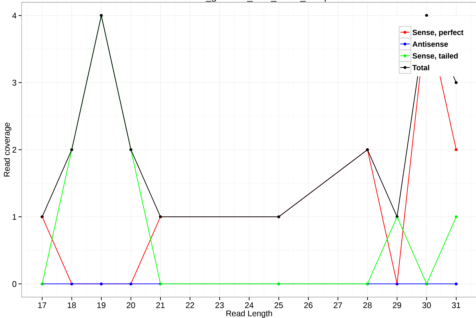
rheMac3_genscan_chr3_91.16_10.5p
