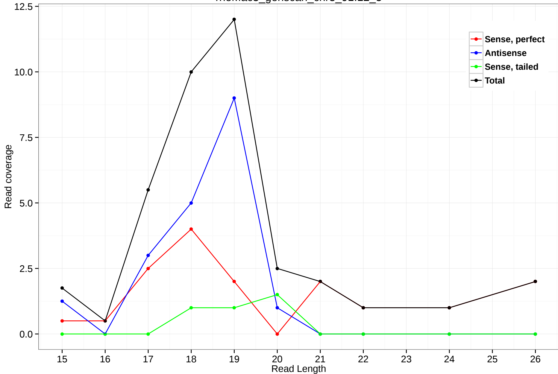
rheMac3_genscan_chr3_91.12_5
