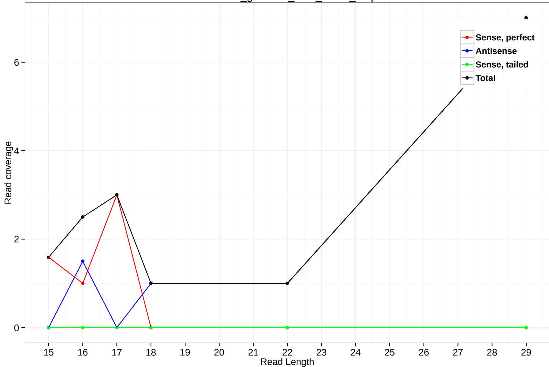
rheMac3_genscan_chr3_91.10_0.5p
