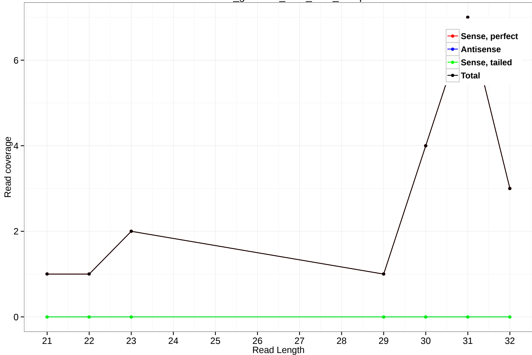
rheMac3_genscan_chr3_87.3_16.5p
