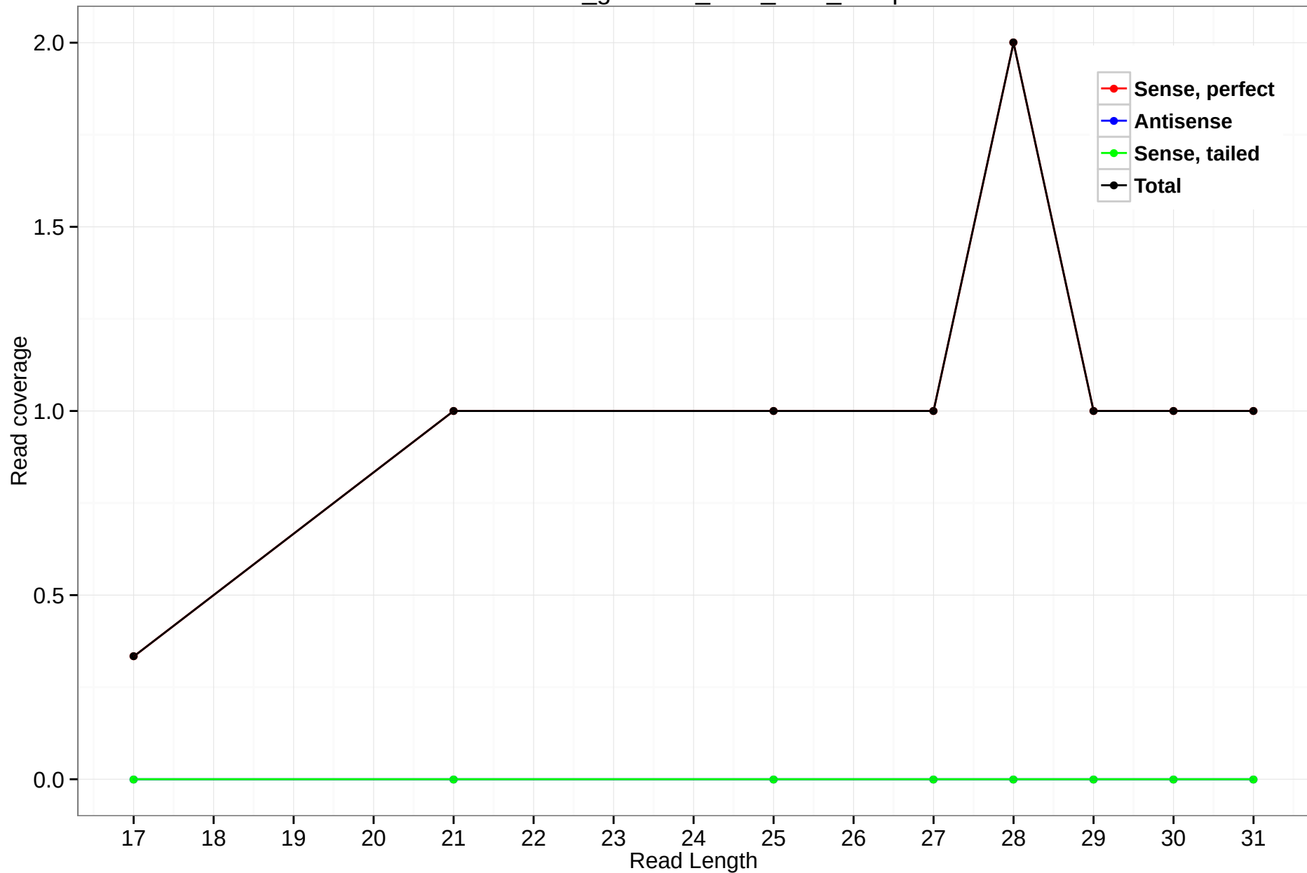
rheMac3_genscan_chr3_87.3_14.5p
