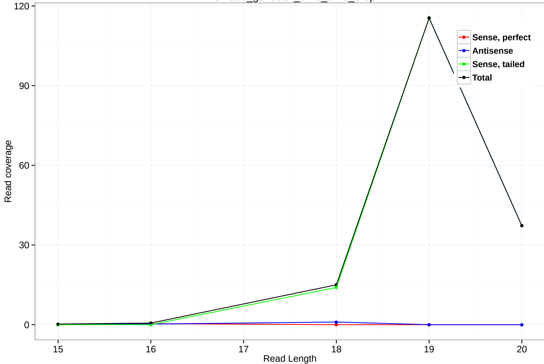
rheMac3_genscan_chr3_82.5_9.3p
