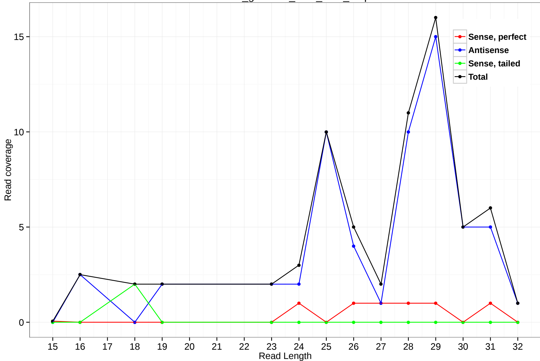
rheMac3_genscan_chr3_82.2_1.3p
