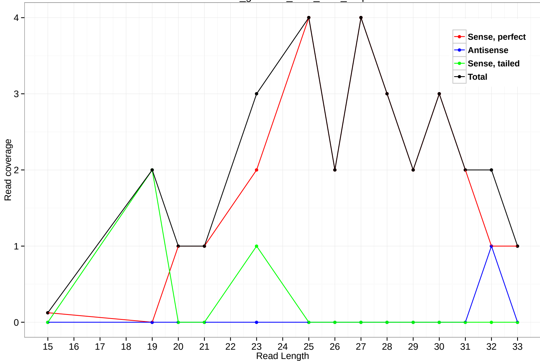
rheMac3_genscan_chr3_66.9_7.5p
