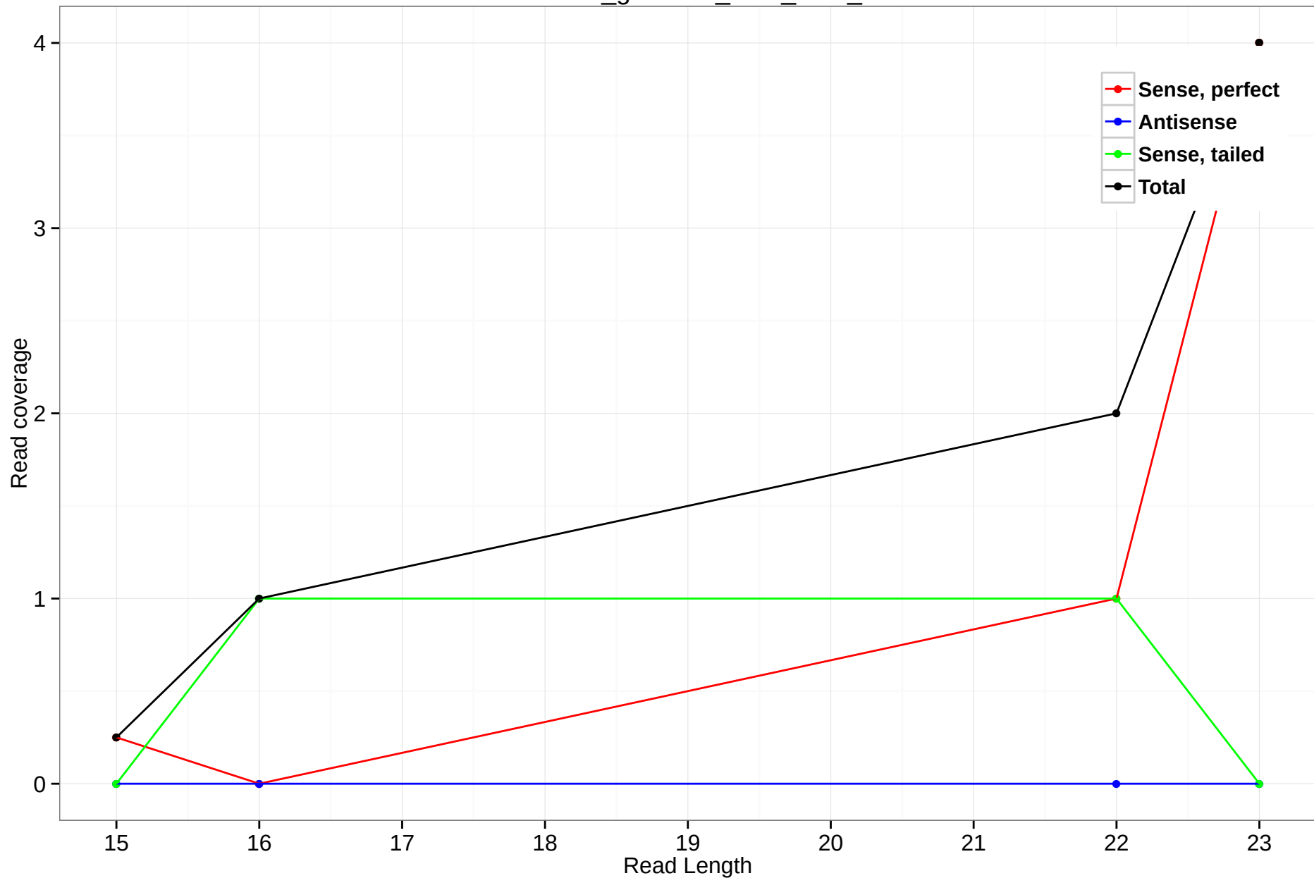
rheMac3_genscan_chr3_66.4_3
