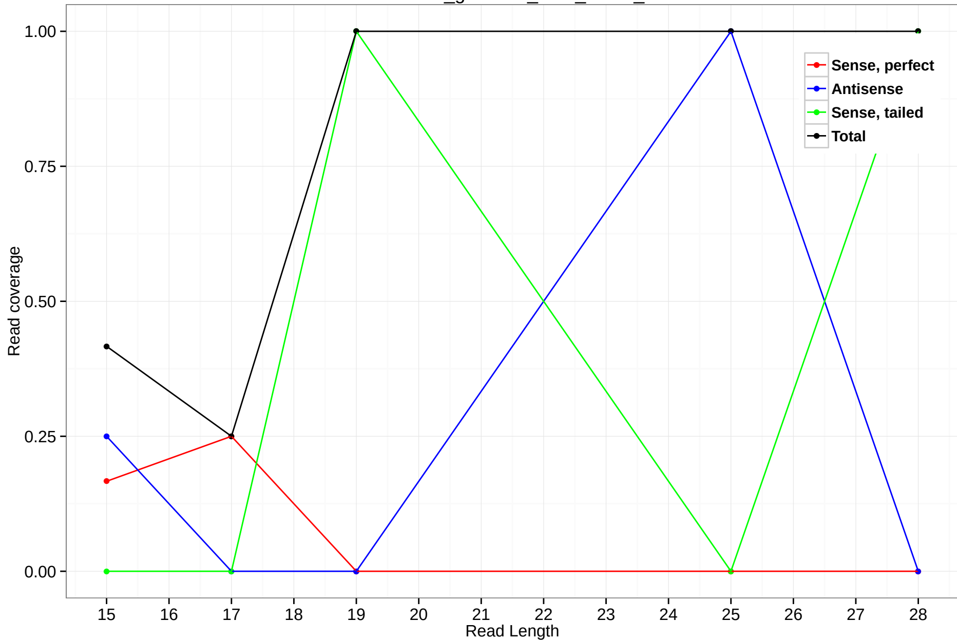
rheMac3_genscan_chr3_65.61_7
