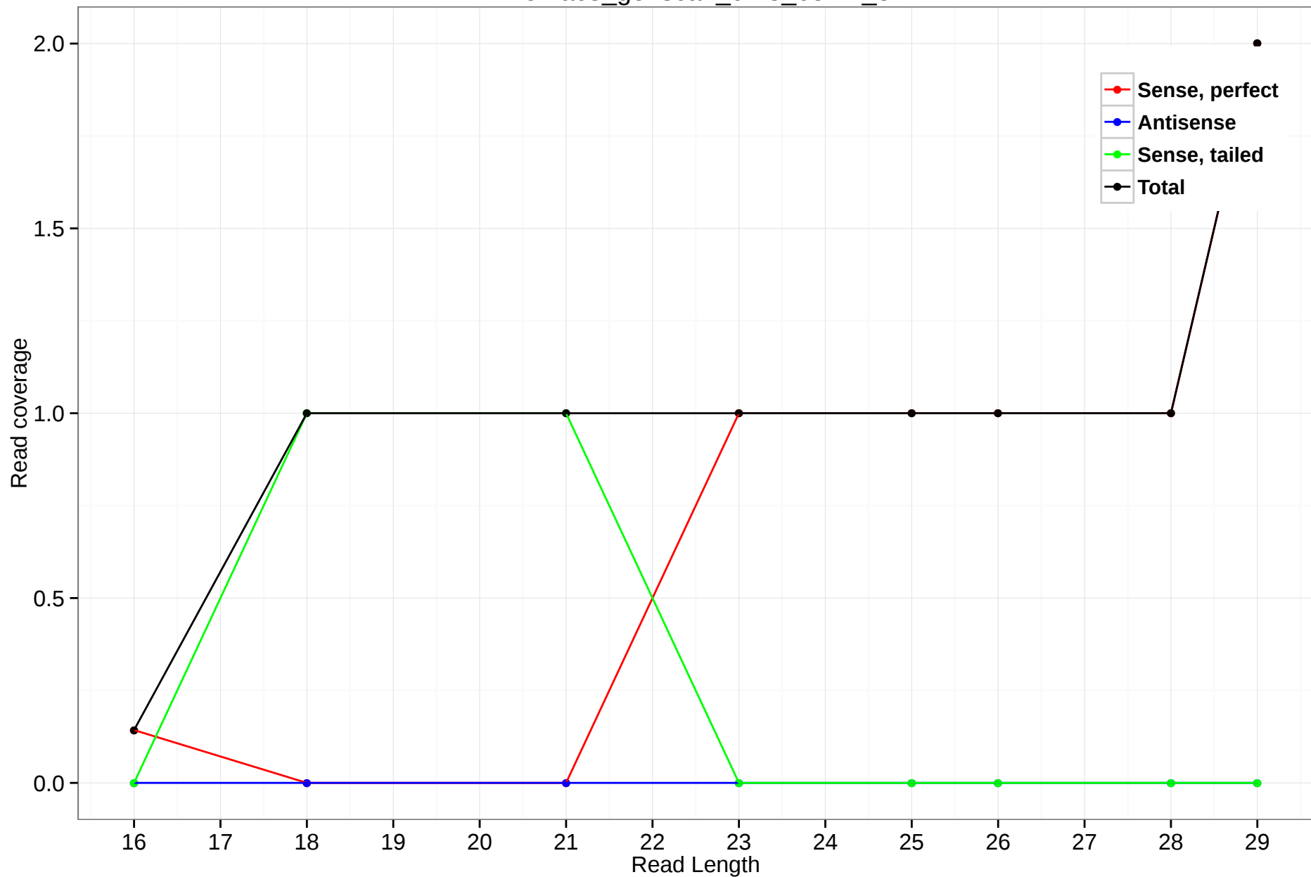
rheMac3_genscan_chr3_65.27_3
