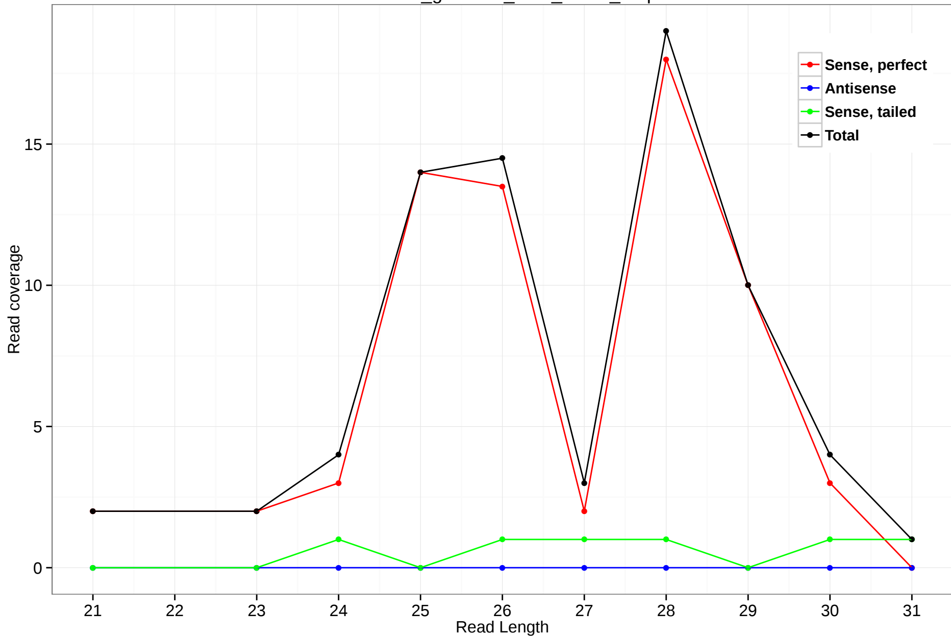
rheMac3_genscan_chr3_65.18_4.5p
