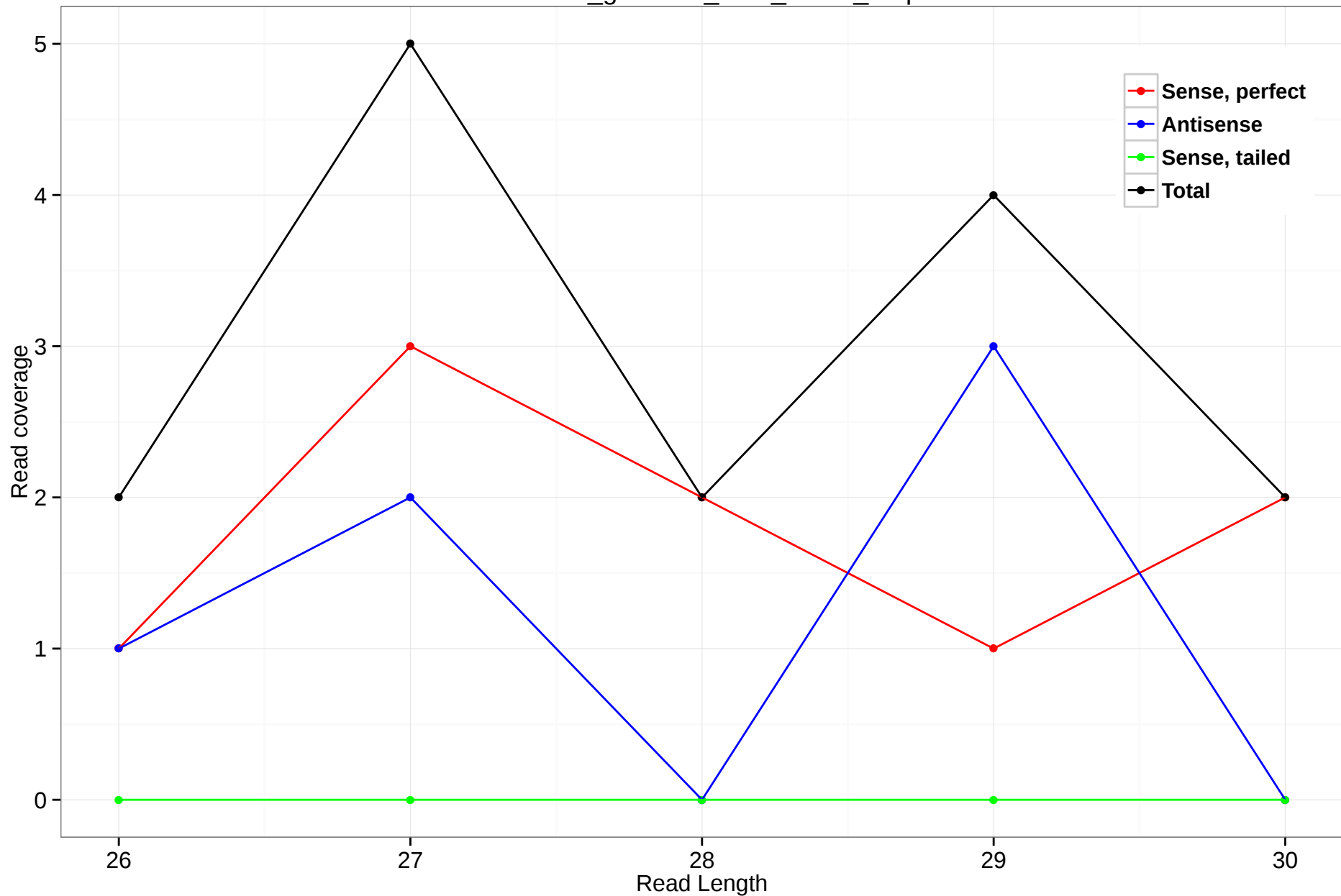
rheMac3_genscan_chr3_65.16_2.3p
